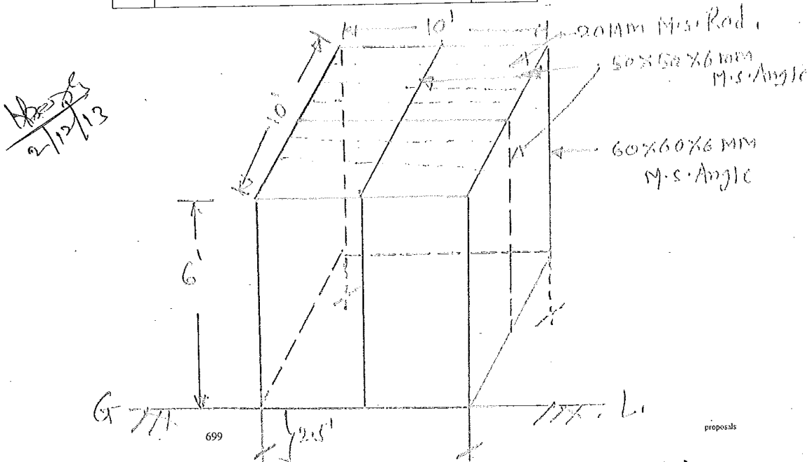
Details of 5000 lit Overhead Sintex Tank platform
